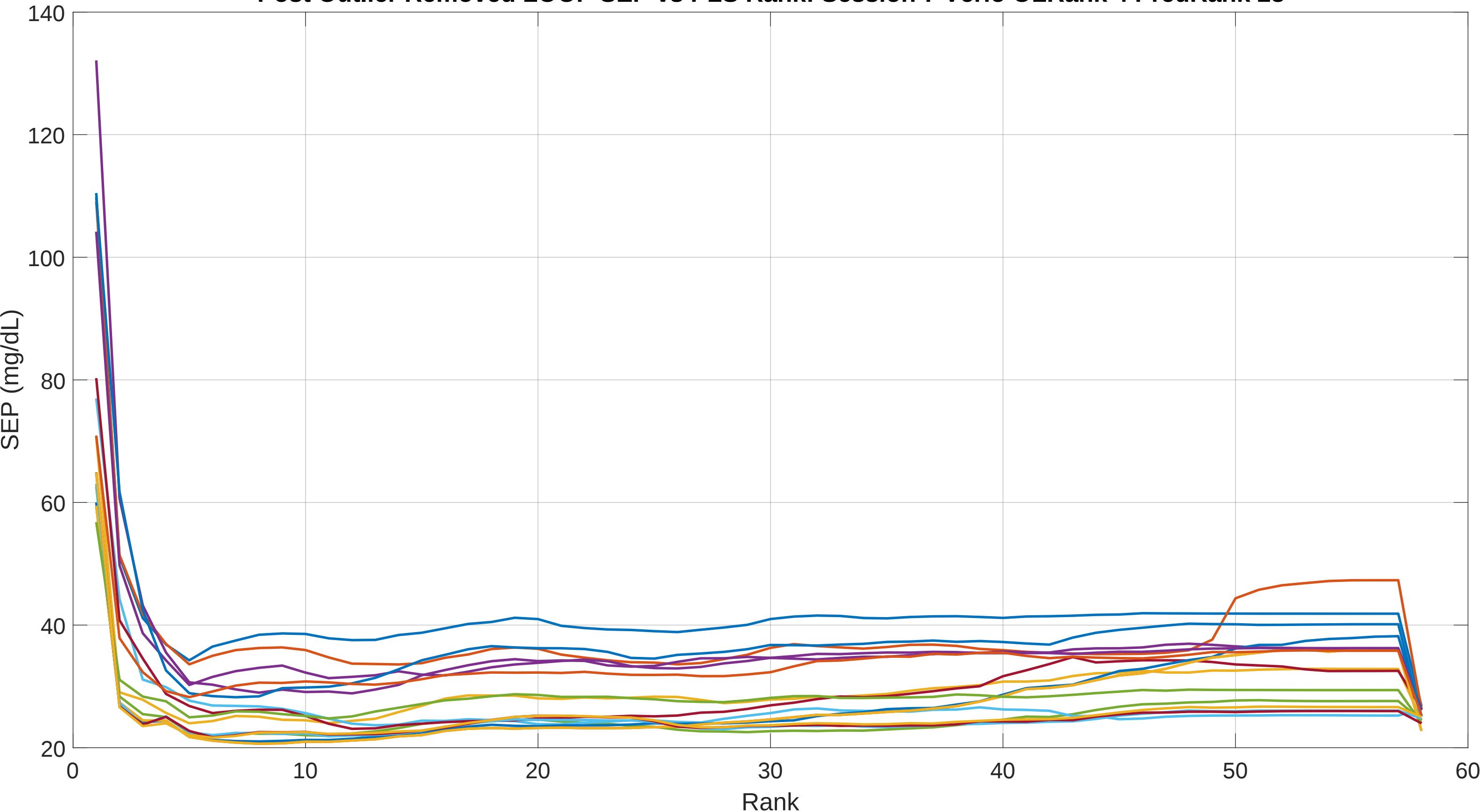
Post Outlier Removed LOOP SEP vs PLS Rank: Session 7 Verio OLRank 4 PredRank 28
