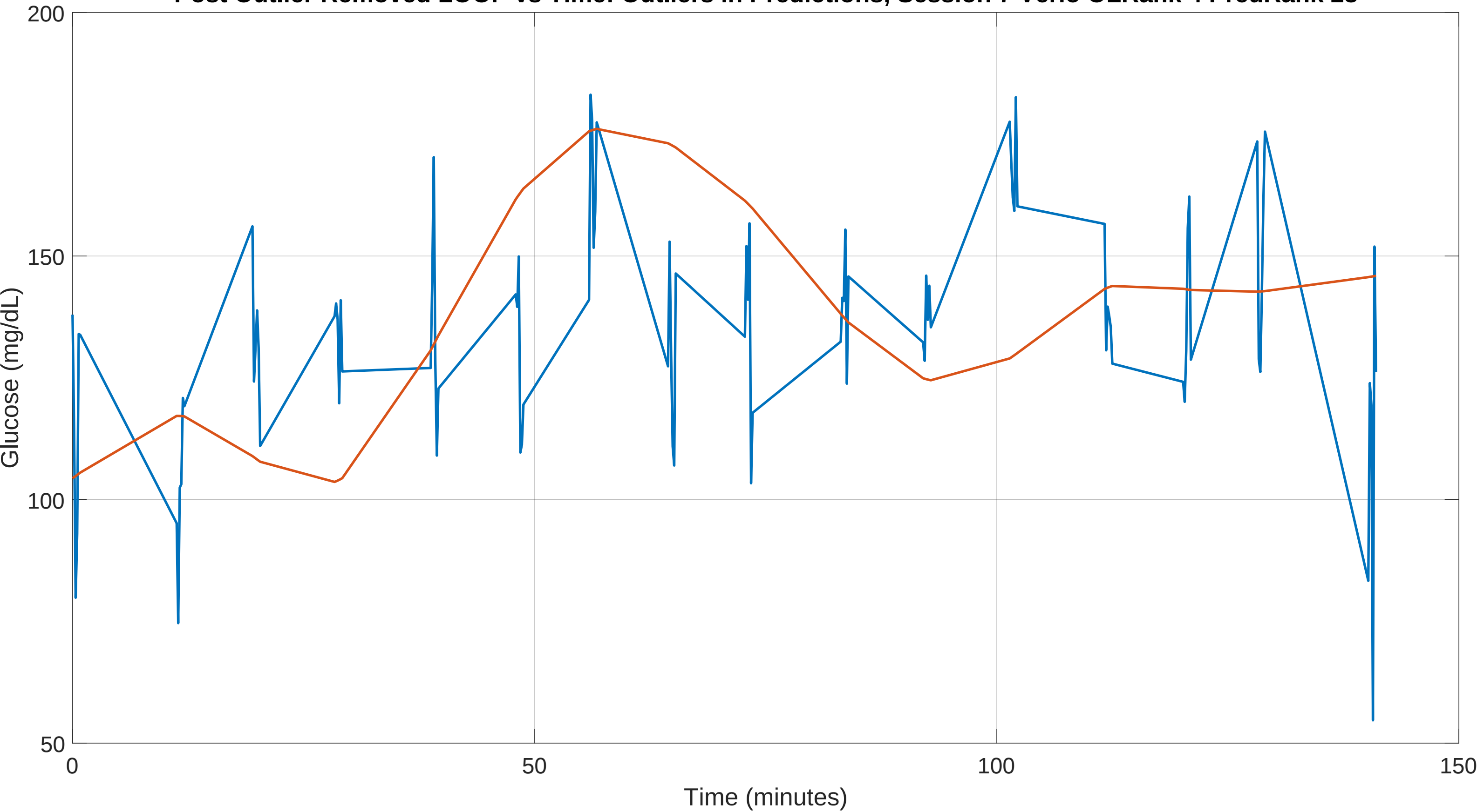
Post Outlier Removed LOOP vs Time: Outliers in Predictions, Session 7 Verio OLRank 4 PredRank 28
