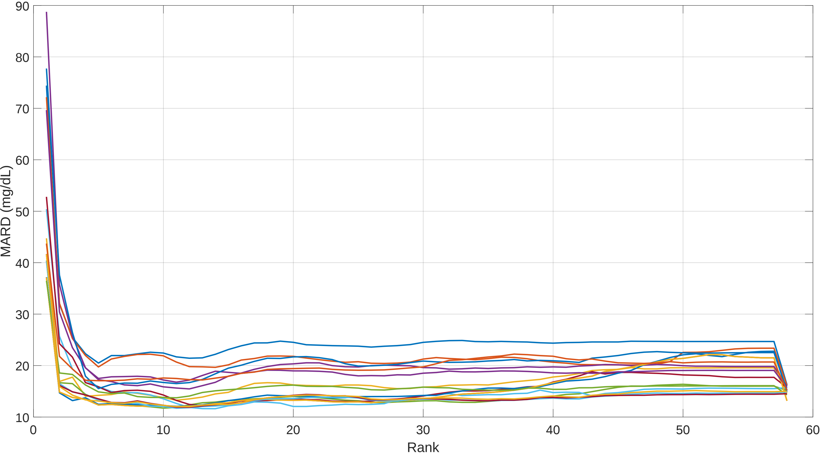
Post Outlier Removed LOOP MARD vs PLS Rank: Session 7 Verio OLRank 4 PredRank 28
