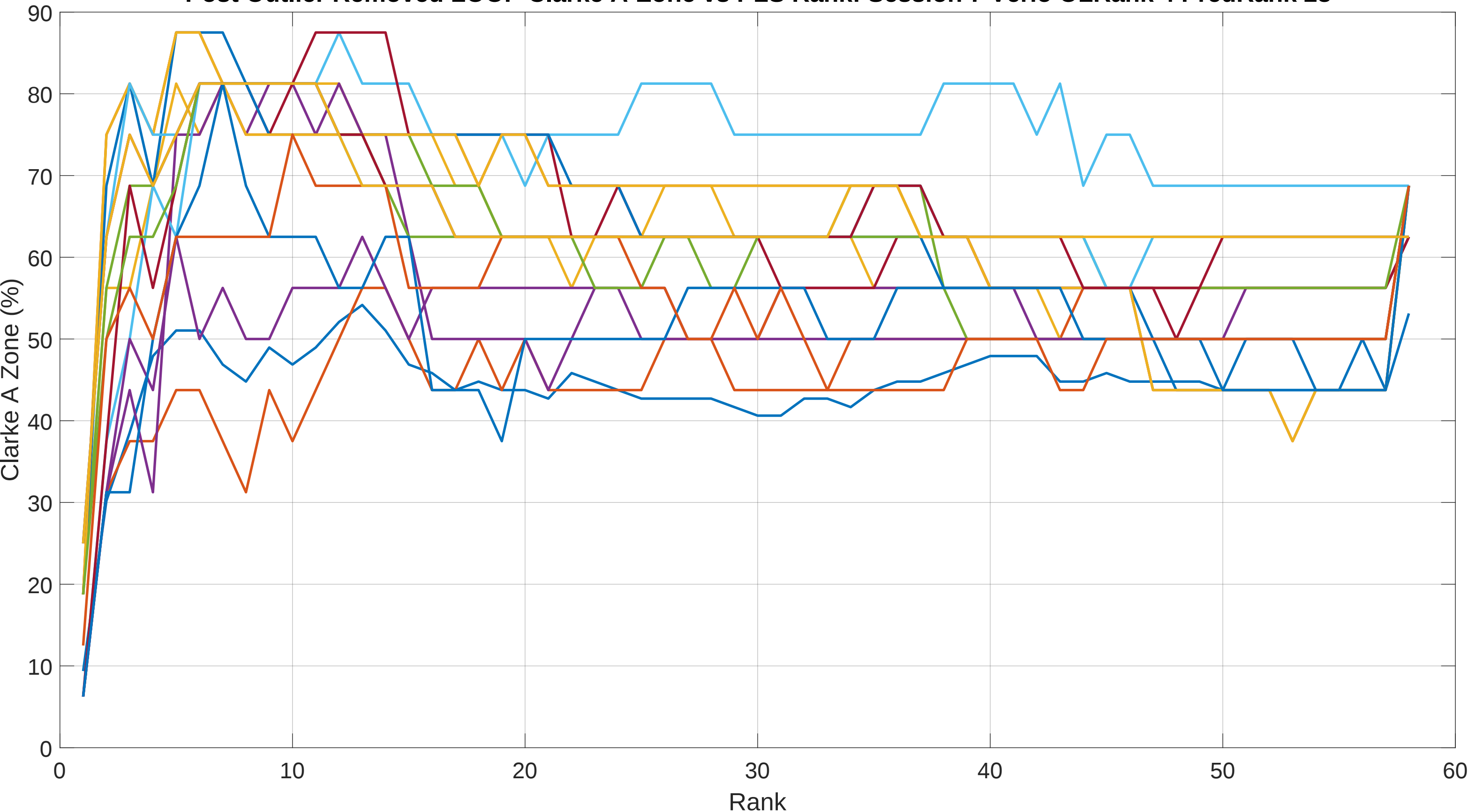
Post Outlier Removed LOOP Clarke A-Zone vs PLS Rank: Session 7 Verio OLRank 4 PredRank 28
