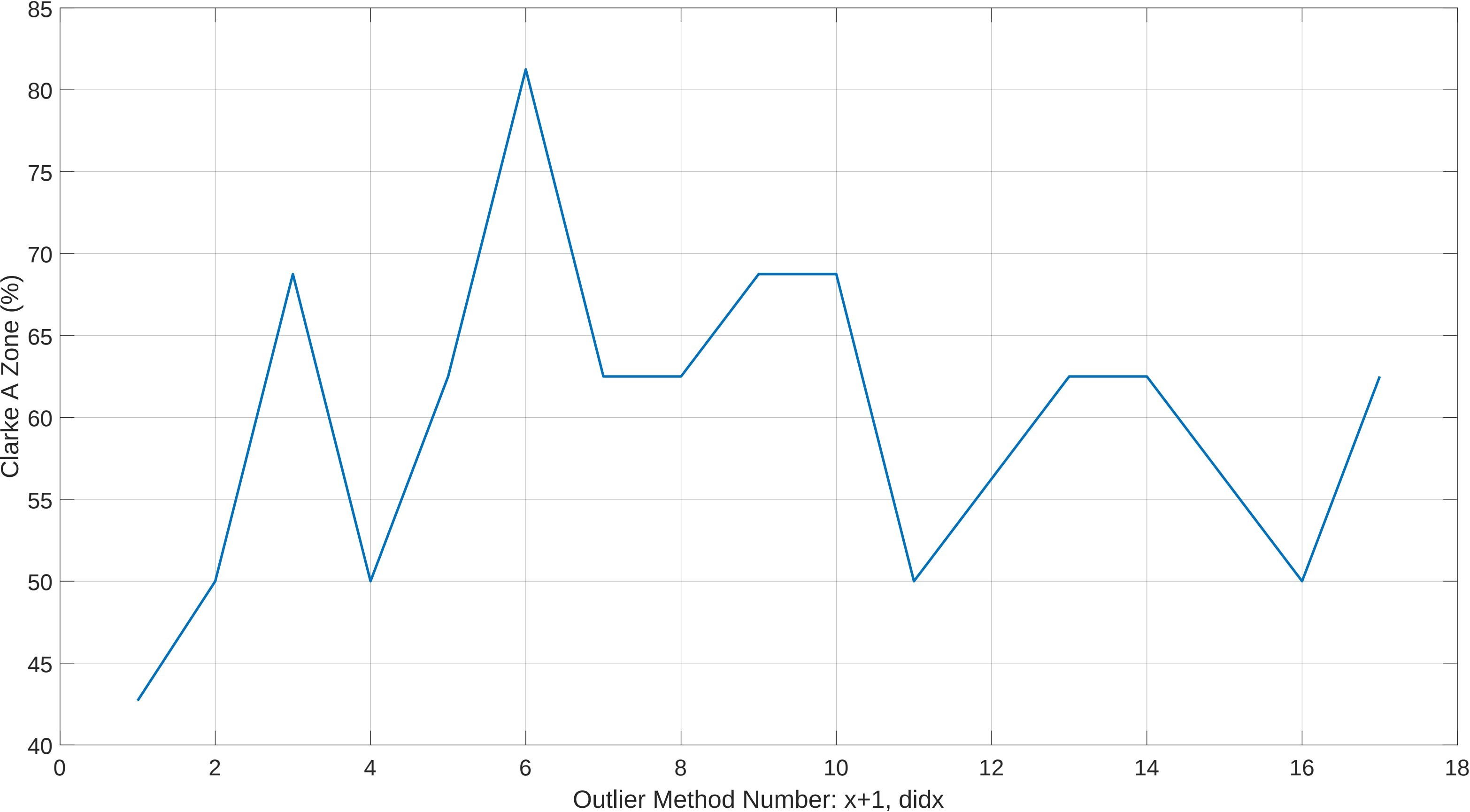
Post Outlier Removed LOOP Clarke A-Zone vs Outlier Method #: Session 7 Verio OLRank 4 PredRank 28
