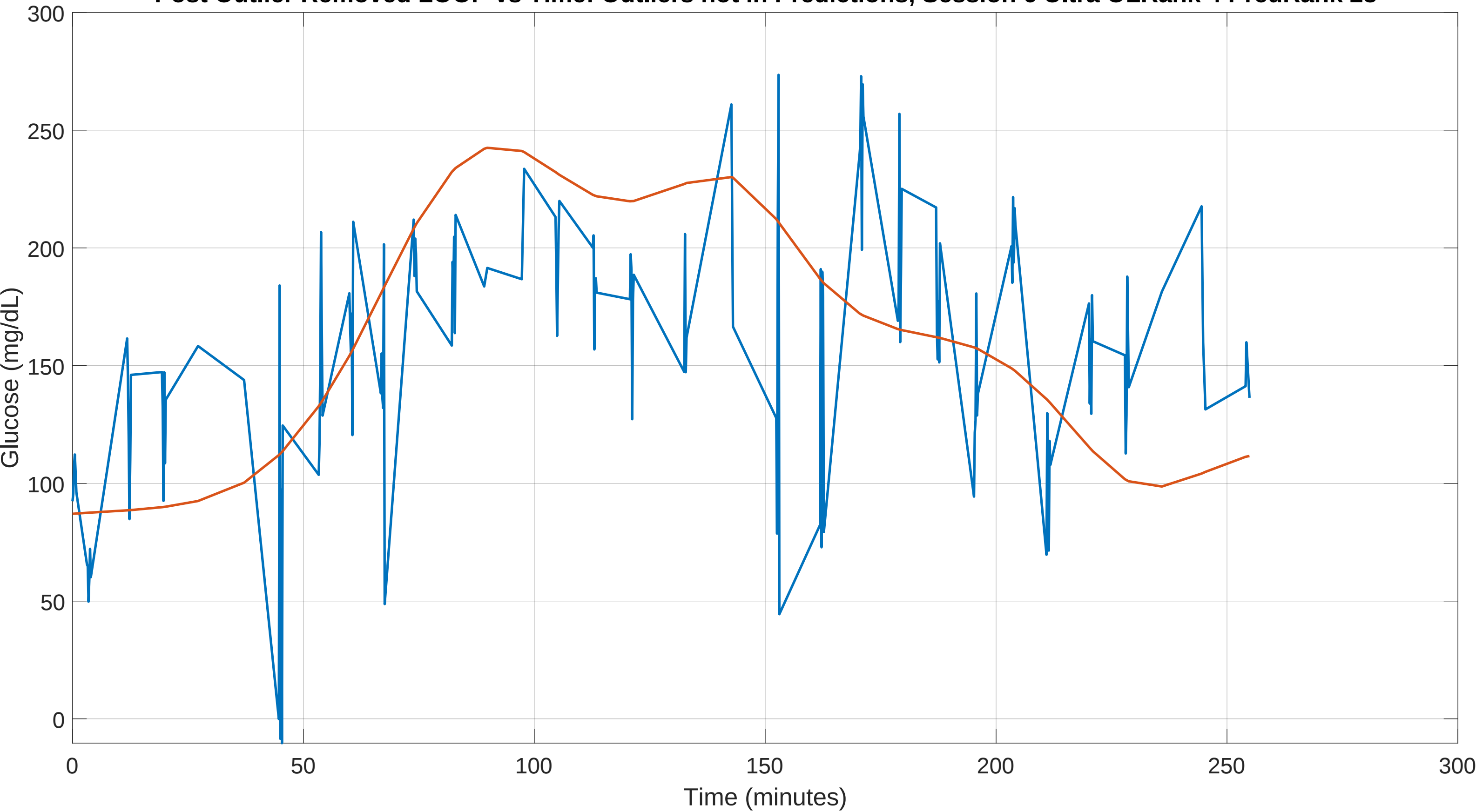
Post Outlier Removed LOOP vs Time: Outliers not in Predictions, Session 6 Ultra OLRank 4 PredRank 28
