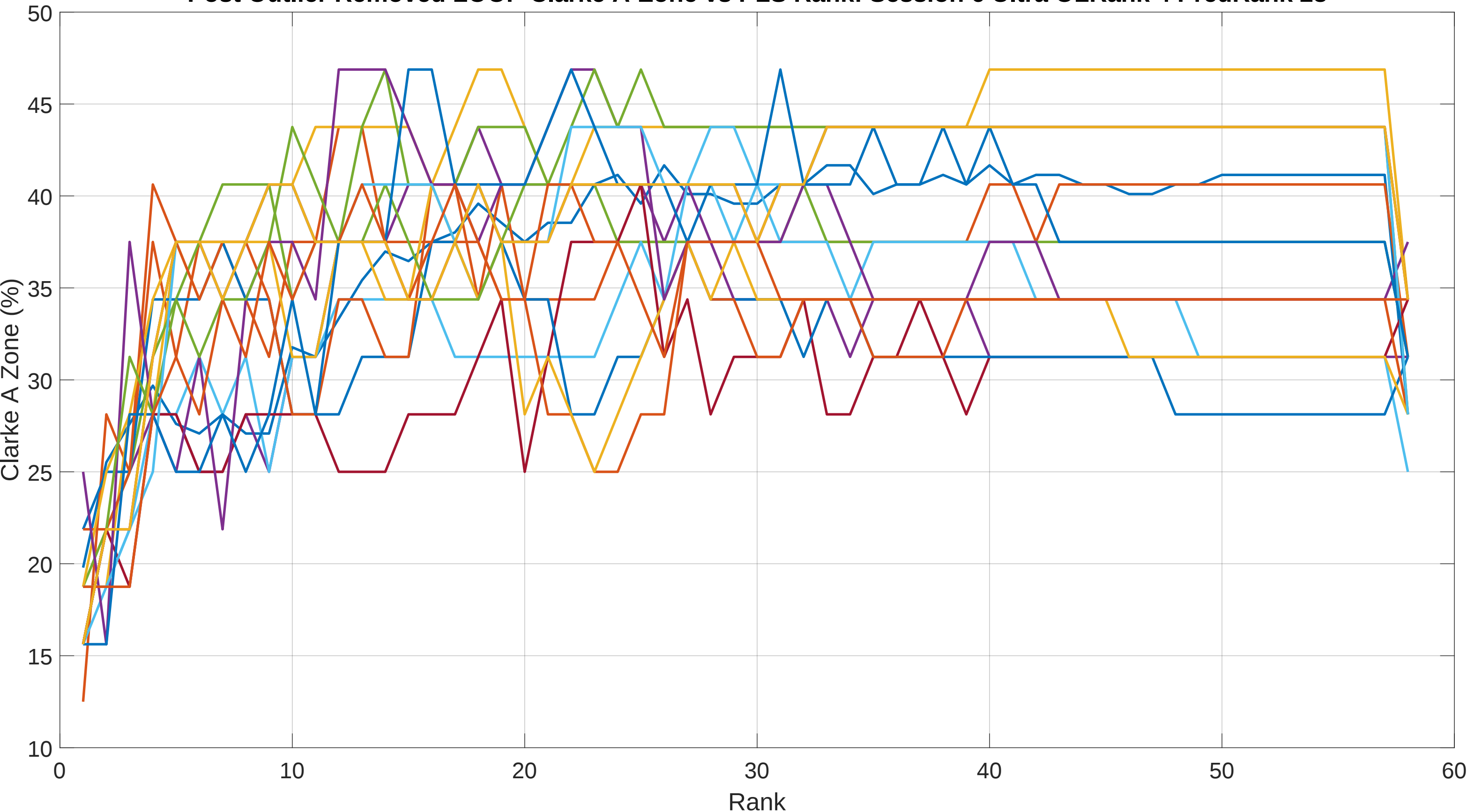
Post Outlier Removed LOOP Clarke A-Zone vs PLS Rank: Session 6 Ultra OLRank 4 PredRank 28
