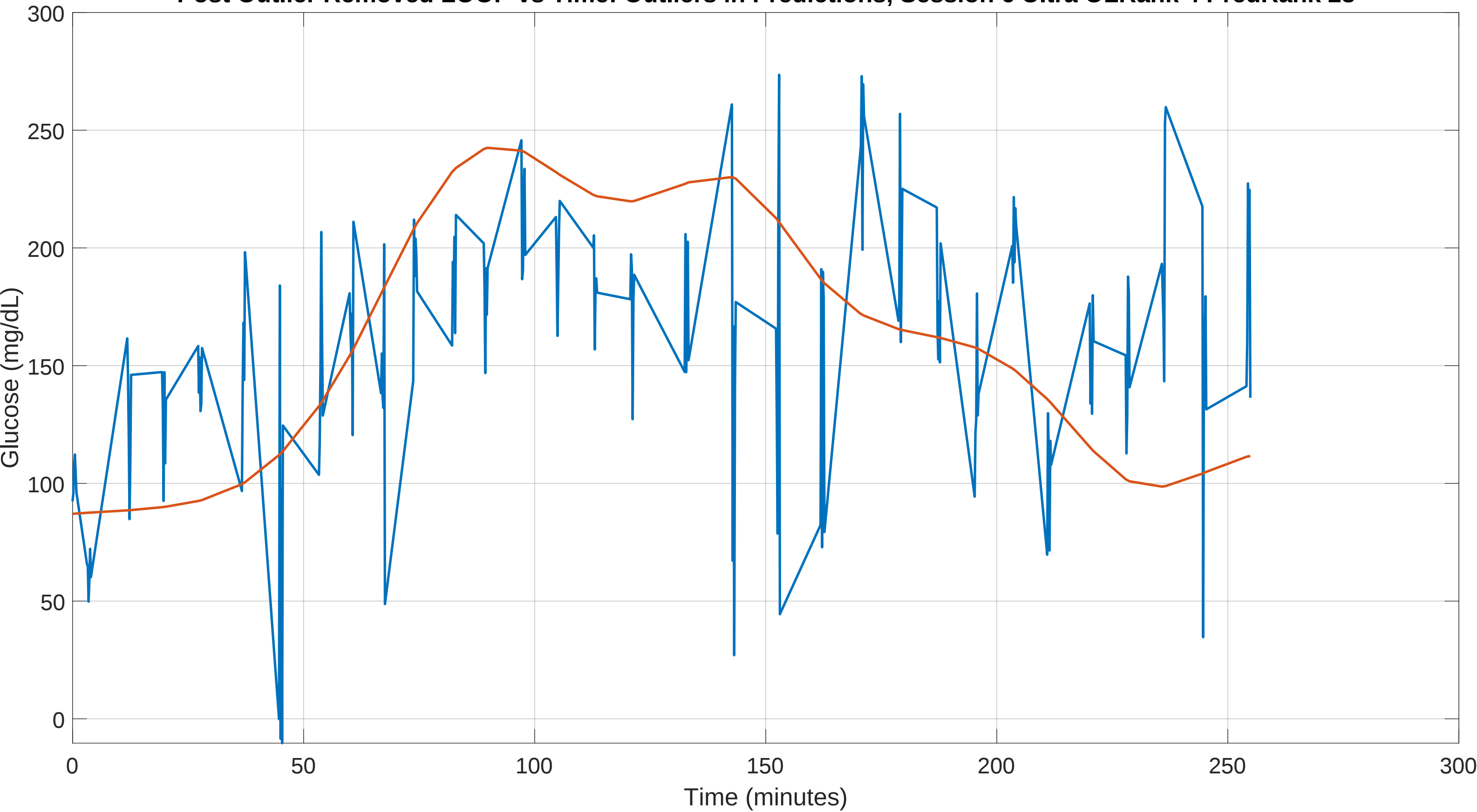
Post Outlier Removed LOOP vs Time: Outliers in Predictions, Session 6 Ultra OLRank 4 PredRank 28
