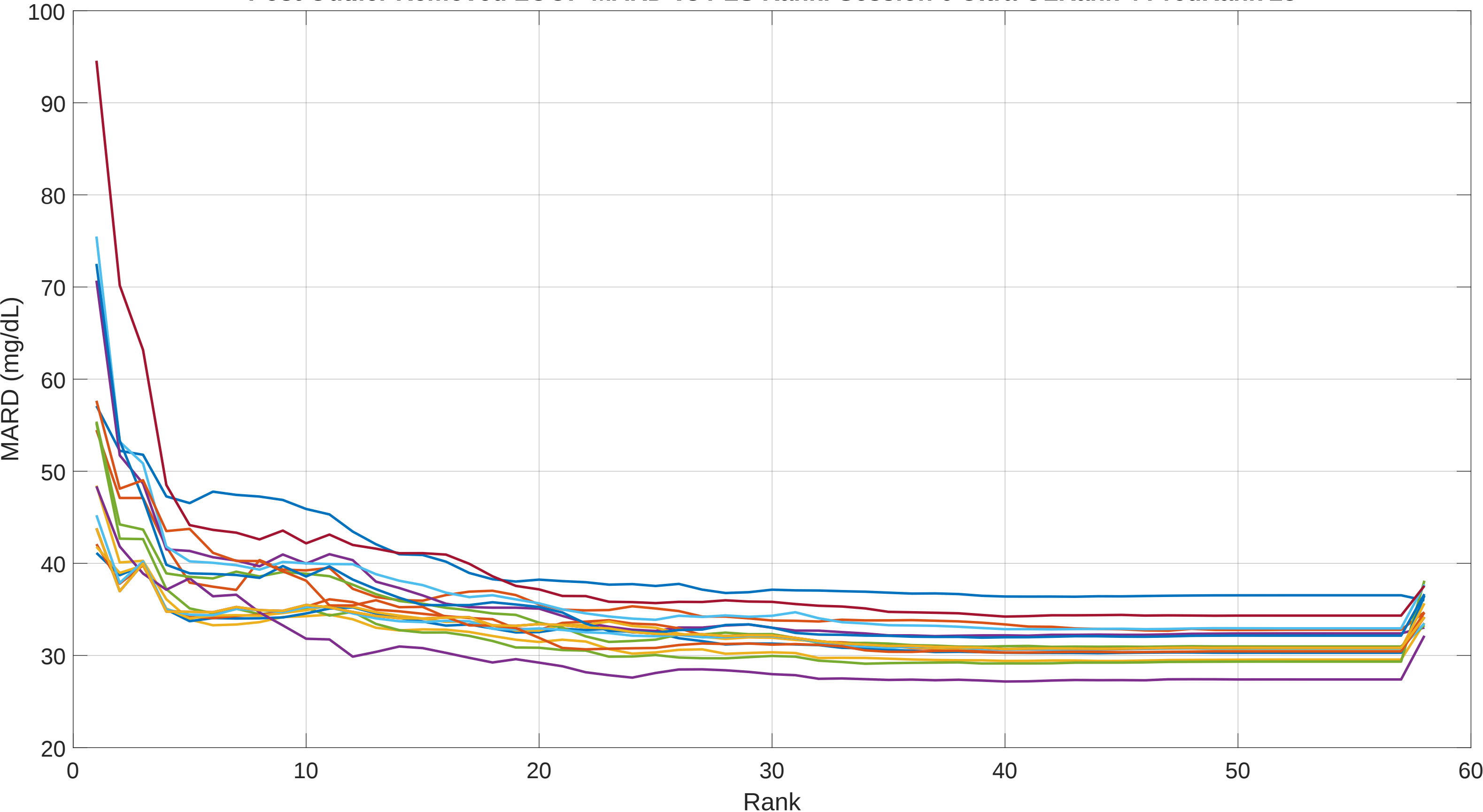
Post Outlier Removed LOOP MARD vs PLS Rank: Session 6 Ultra OLRank 4 PredRank 28
