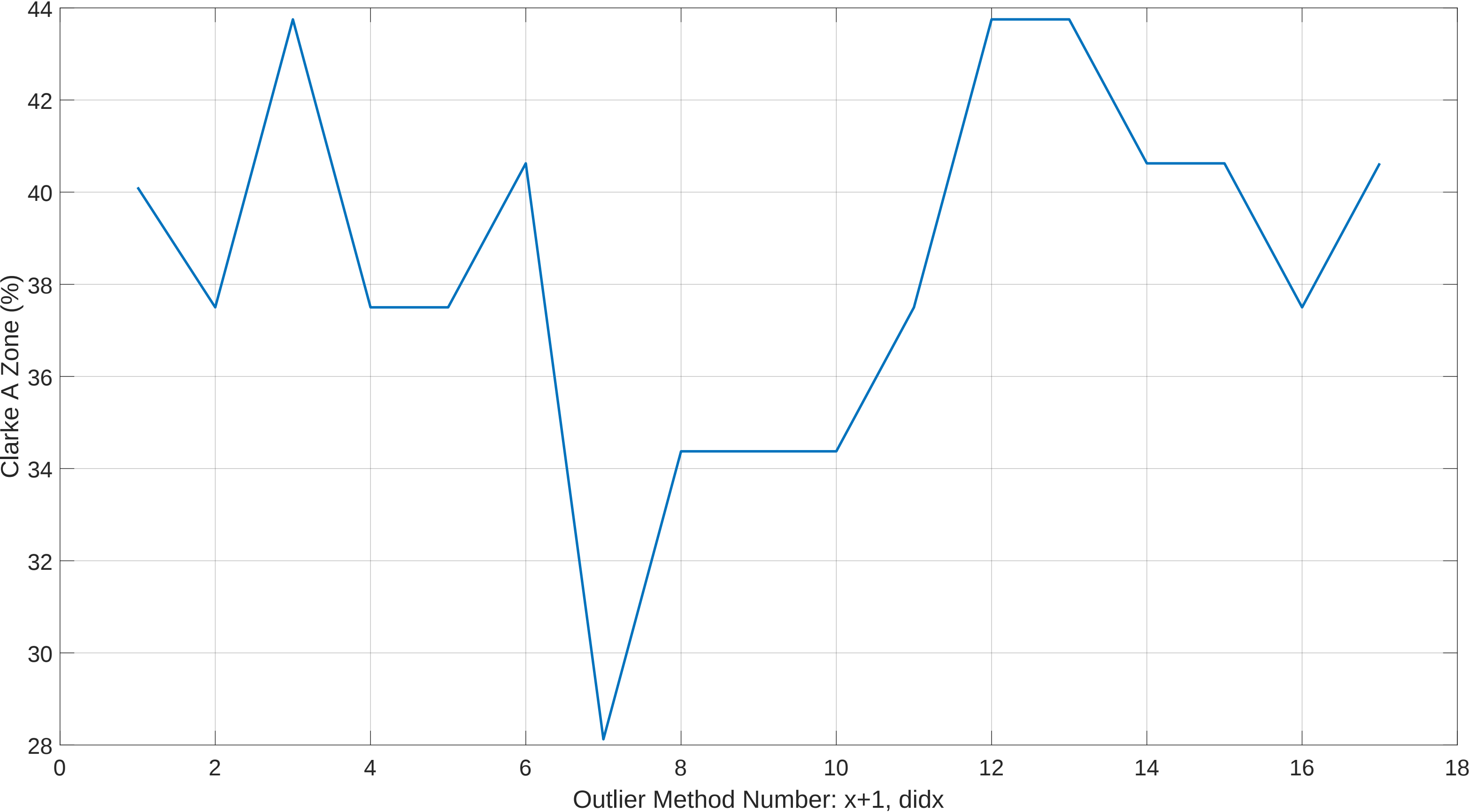
Post Outlier Removed LOOP Clarke A-Zone vs Outlier Method #: Session 6 Ultra OLRank 4 PredRank 28
