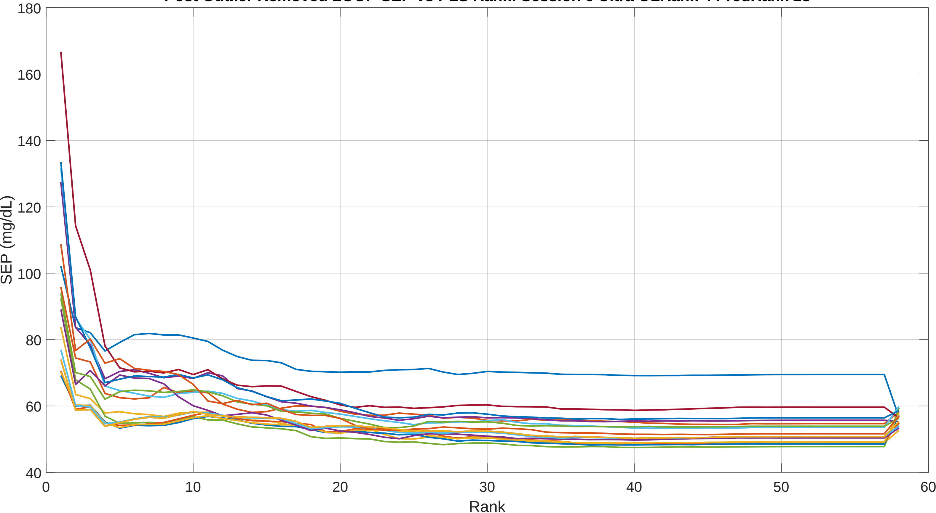
Post Outlier Removed LOOP SEP vs PLS Rank: Session 6 Ultra OLRank 4 PredRank 28
