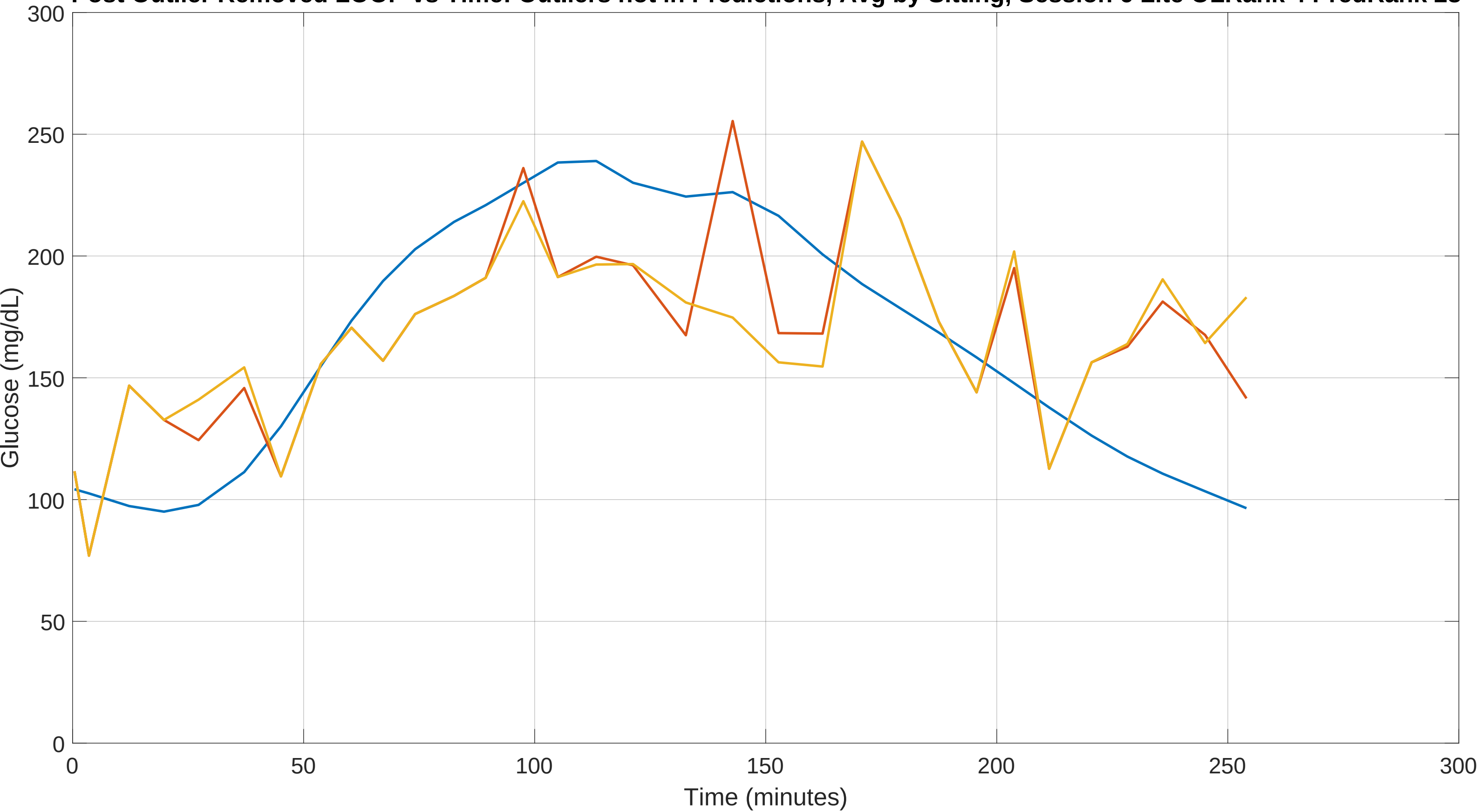
Post Outlier Removed LOOP vs Time: Outliers not in Predictions, Avg by Sitting, Session 6 Lite OLRank 4 PredRank 28
