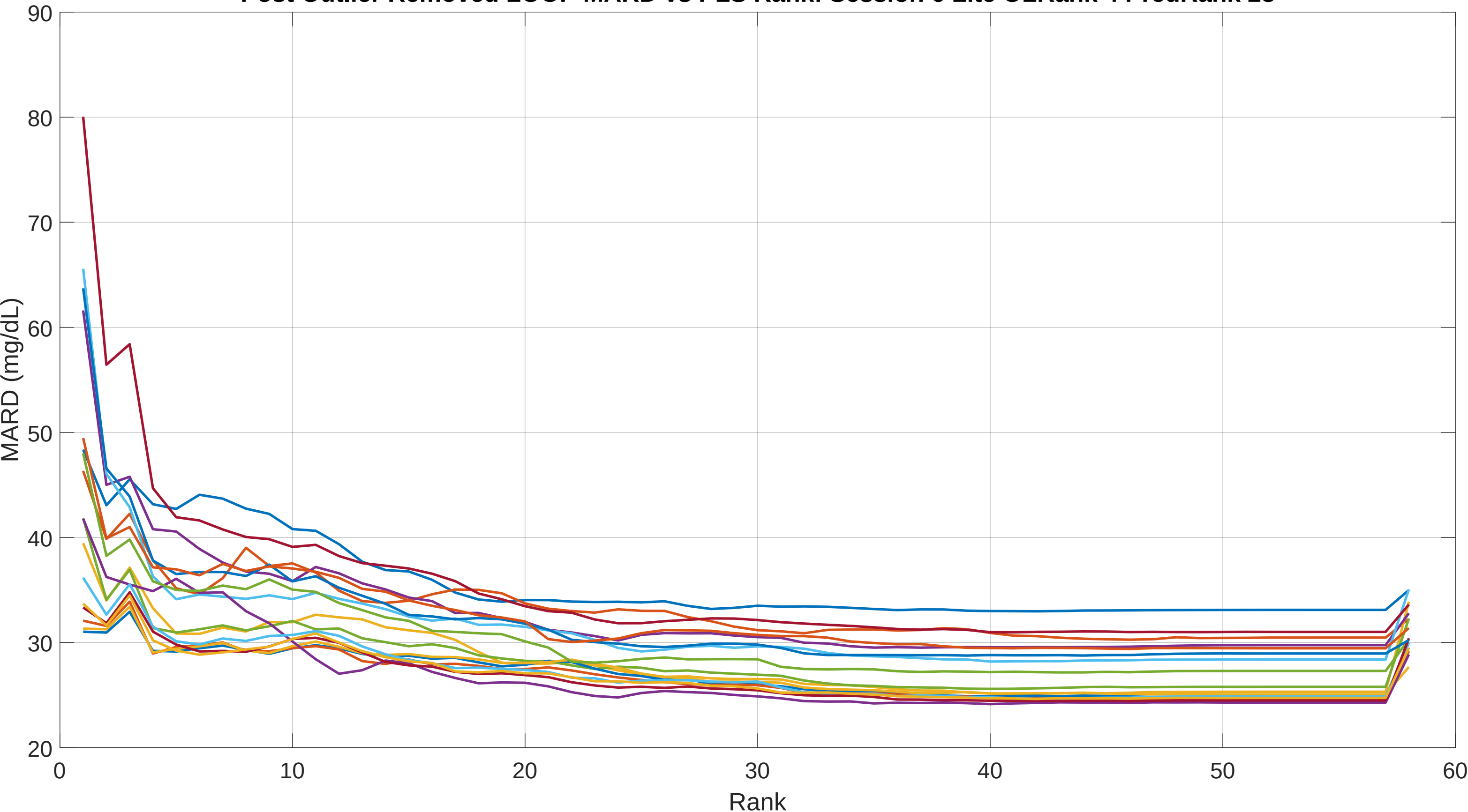
Post Outlier Removed LOOP MARD vs PLS Rank: Session 6 Lite OLRank 4 PredRank 28
