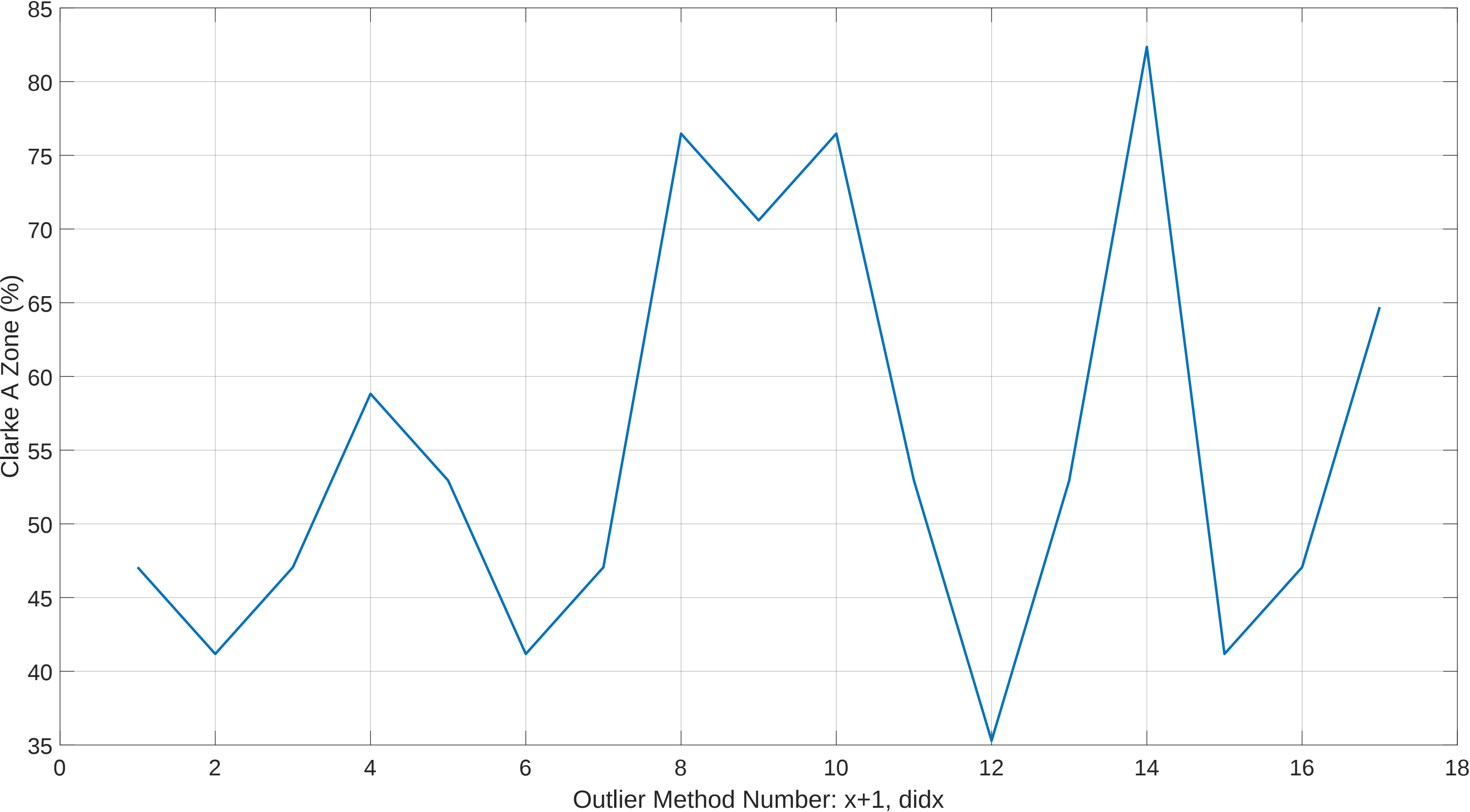
Post Outlier Removed LOOP Clarke A-Zone vs Outlier Method #: Session 5 Ultra OLRank 4 PredRank 28
