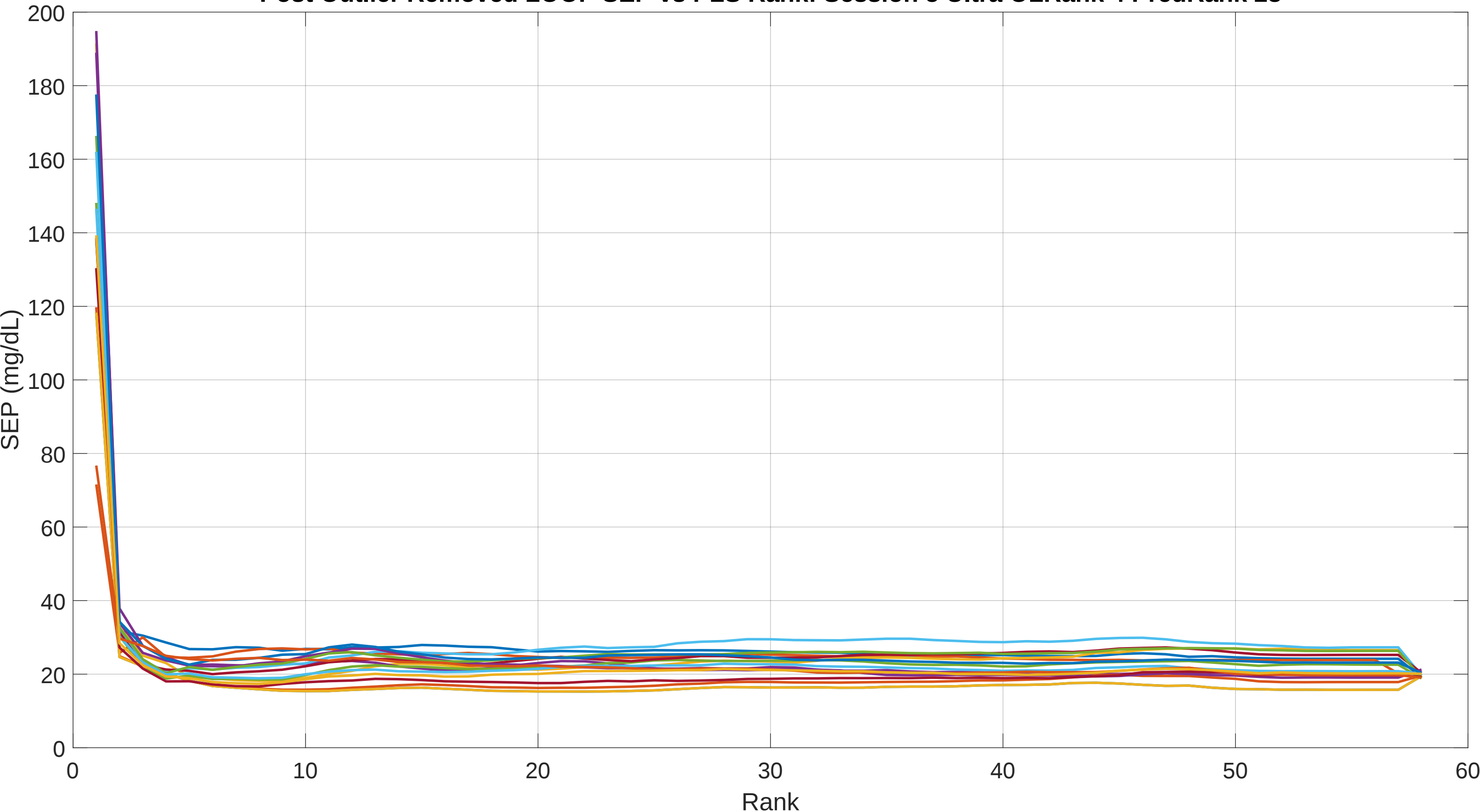
Post Outlier Removed LOOP SEP vs PLS Rank: Session 5 Ultra OLRank 4 PredRank 28
