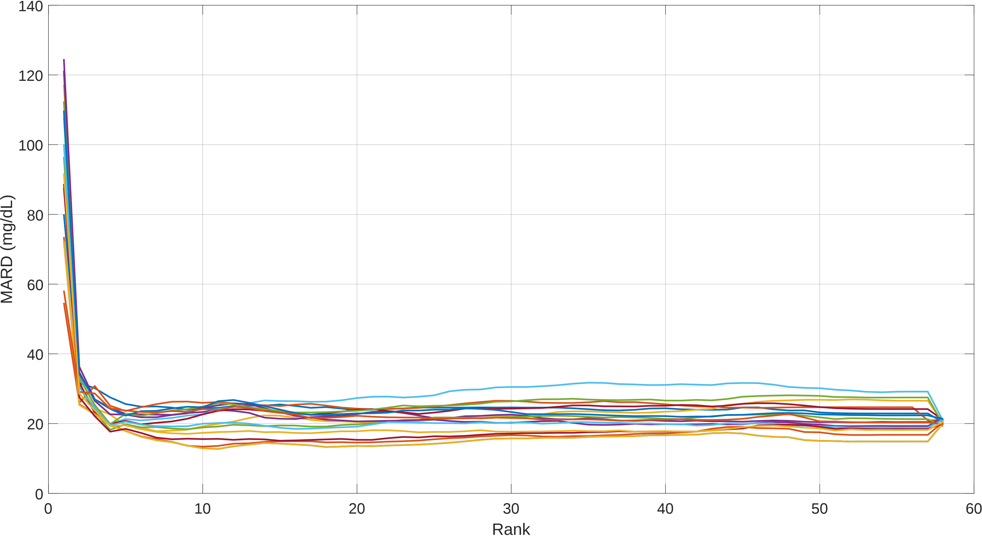
Post Outlier Removed LOOP MARD vs PLS Rank: Session 5 Ultra OLRank 4 PredRank 28
