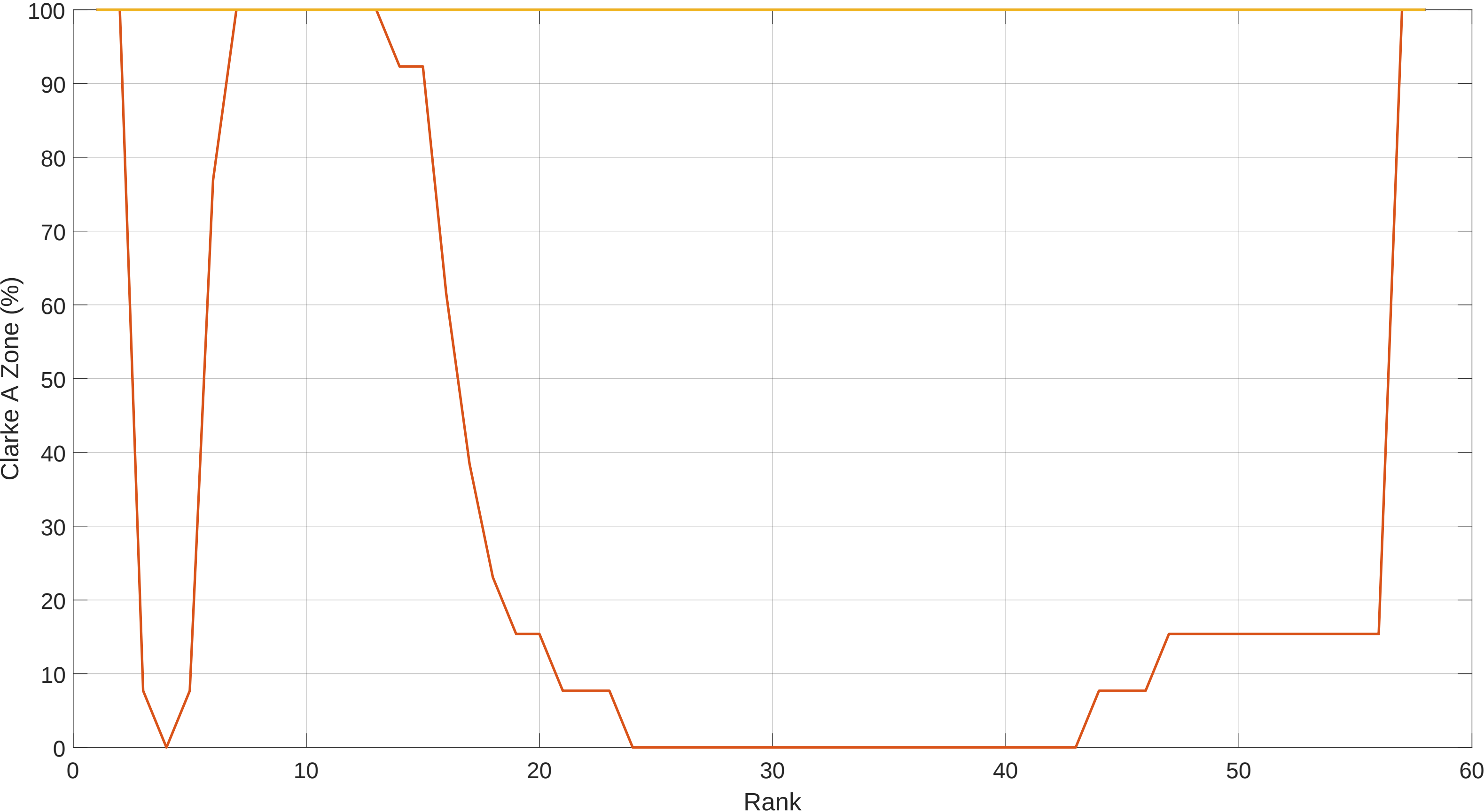
Post Outlier Removed LOOP Clarke A-Zone vs PLS Rank: Session 9 Oxi OLRank 57 PredRank 28
