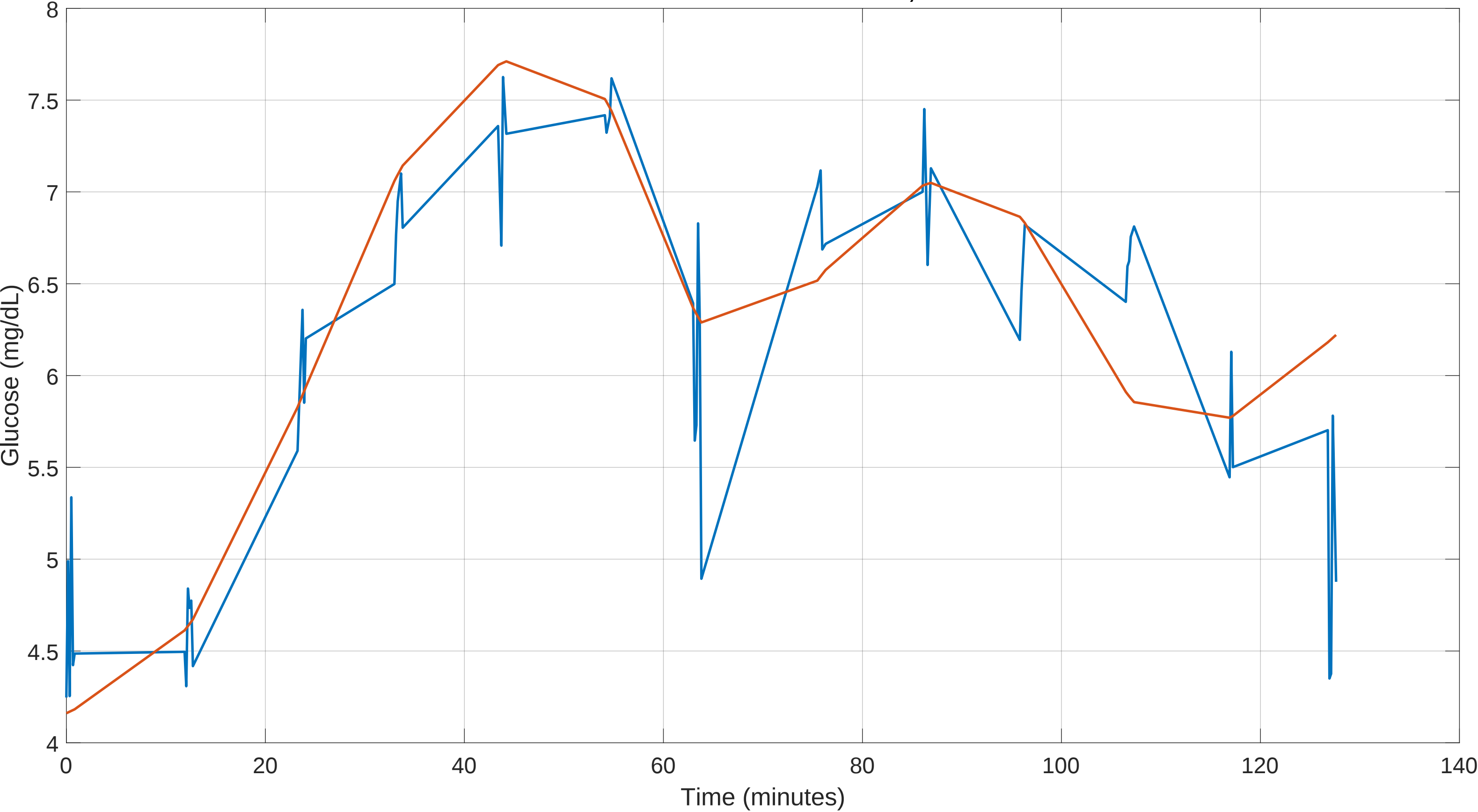
Post Outlier Removed LOOP vs Time: Outliers not in Predictions, Session 9 Oxi OLRank 57 PredRank 28
