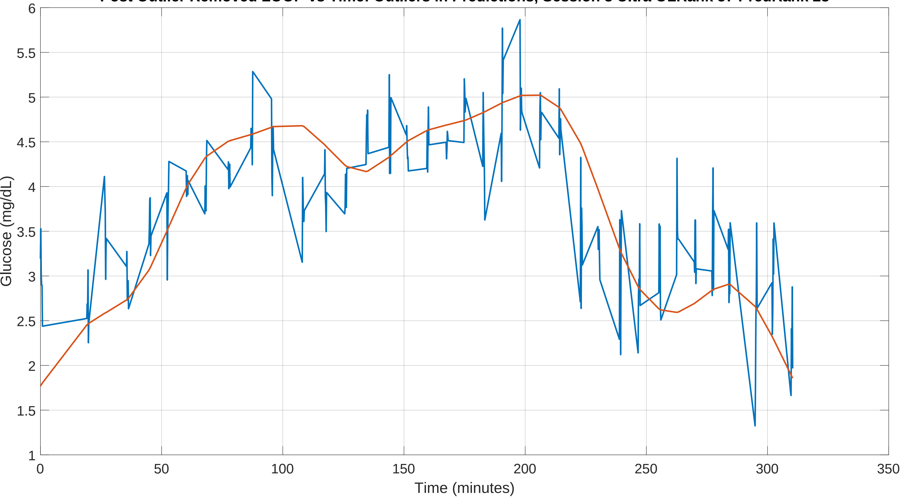
Post Outlier Removed LOOP vs Time: Outliers in Predictions, Session 3 Ultra OLRank 57 PredRank 28
