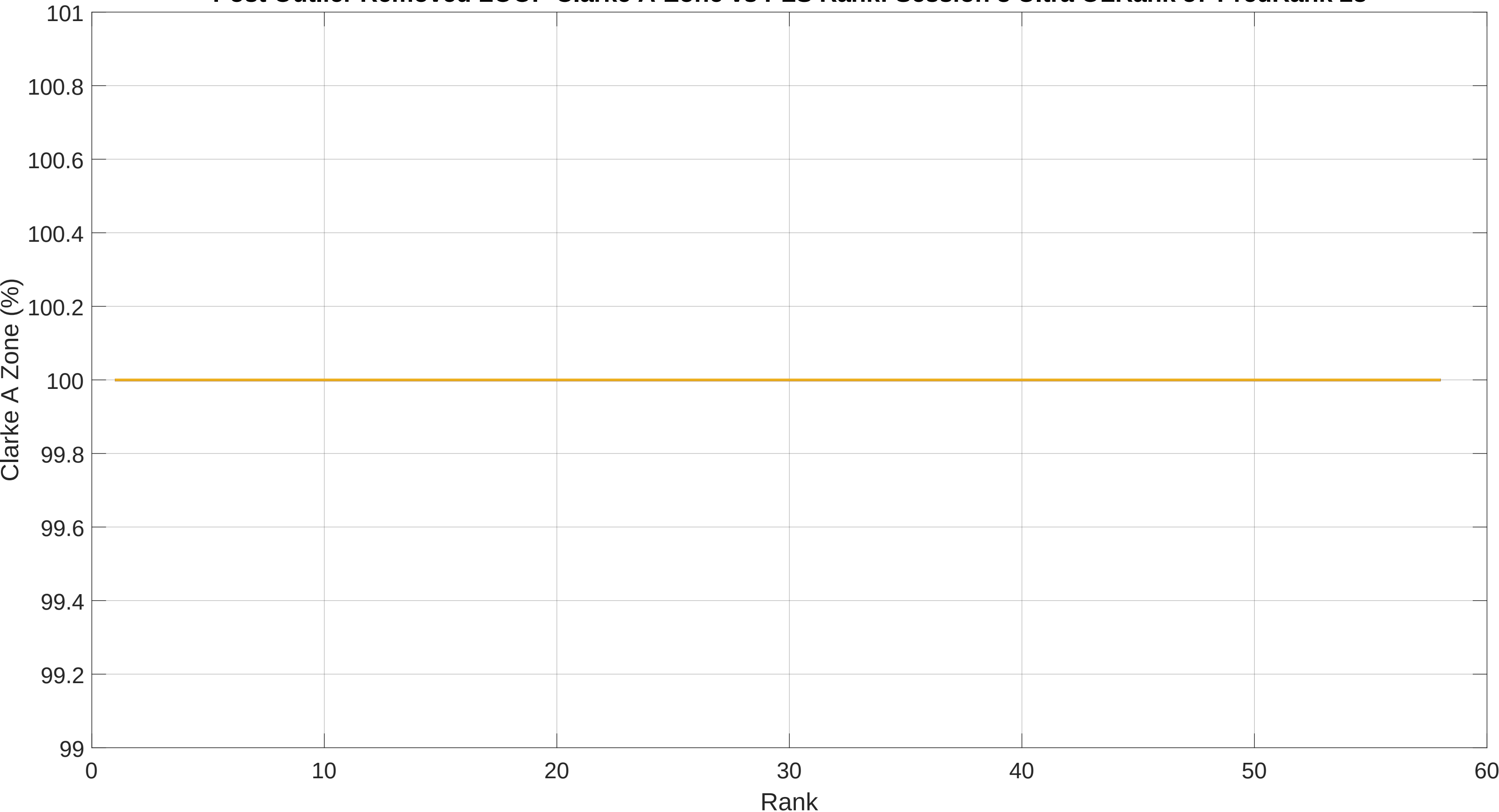
Post Outlier Removed LOOP Clarke A-Zone vs PLS Rank: Session 3 Ultra OLRank 57 PredRank 28
