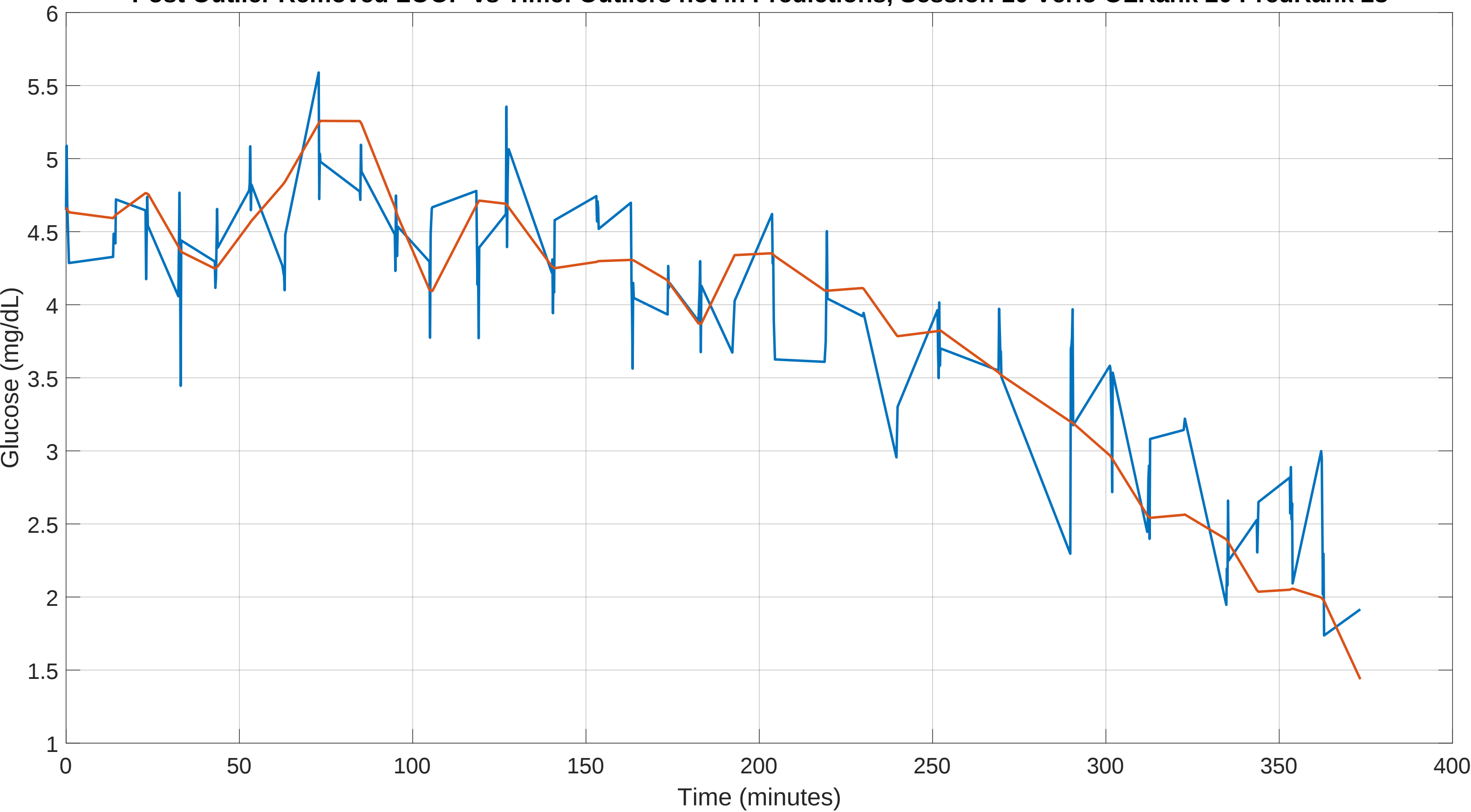
Post Outlier Removed LOOP vs Time: Outliers not in Predictions, Session 10 Verio OLRank 20 PredRank 28
