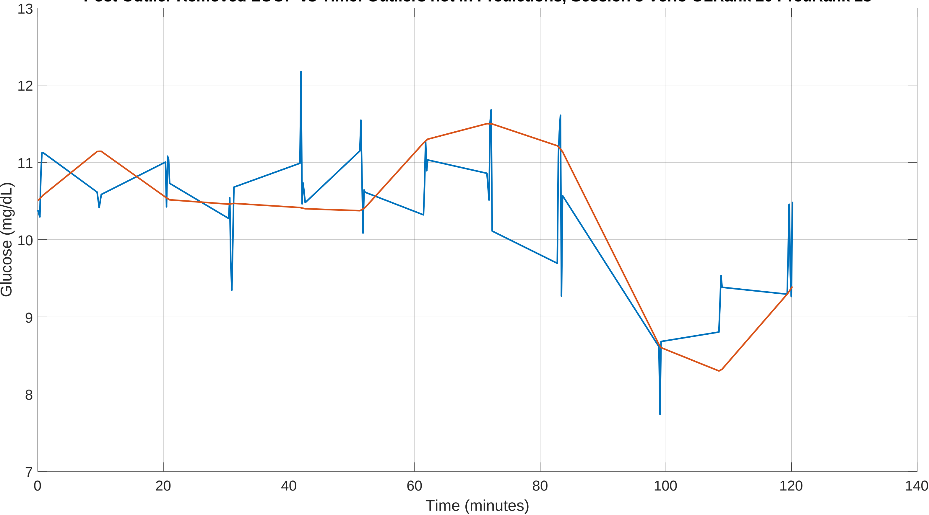
Post Outlier Removed LOOP vs Time: Outliers not in Predictions, Session 8 Verio OLRank 20PredRank 28
