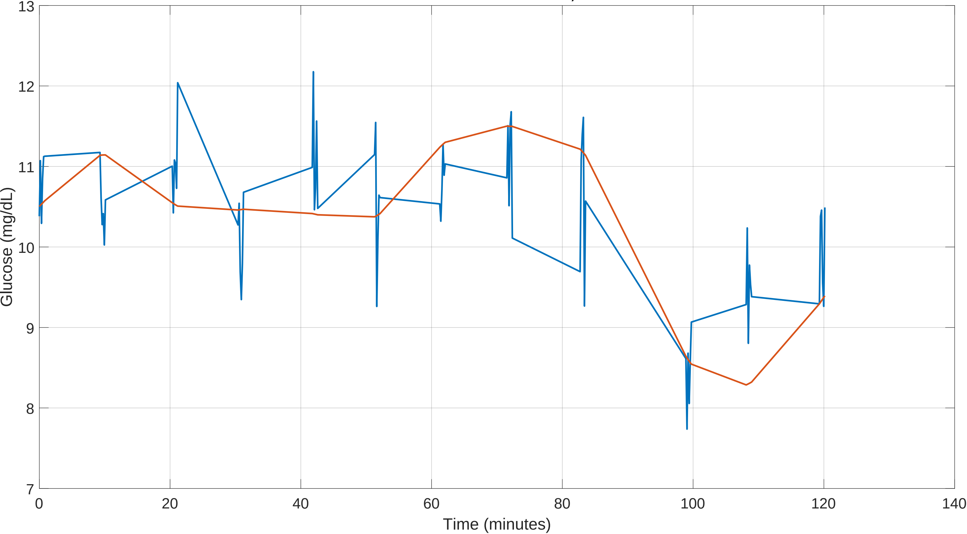
Post Outlier Removed LOOP vs Time: Outliers in Predictions, Session 8 Verio OLRank 20 PredRank 28
