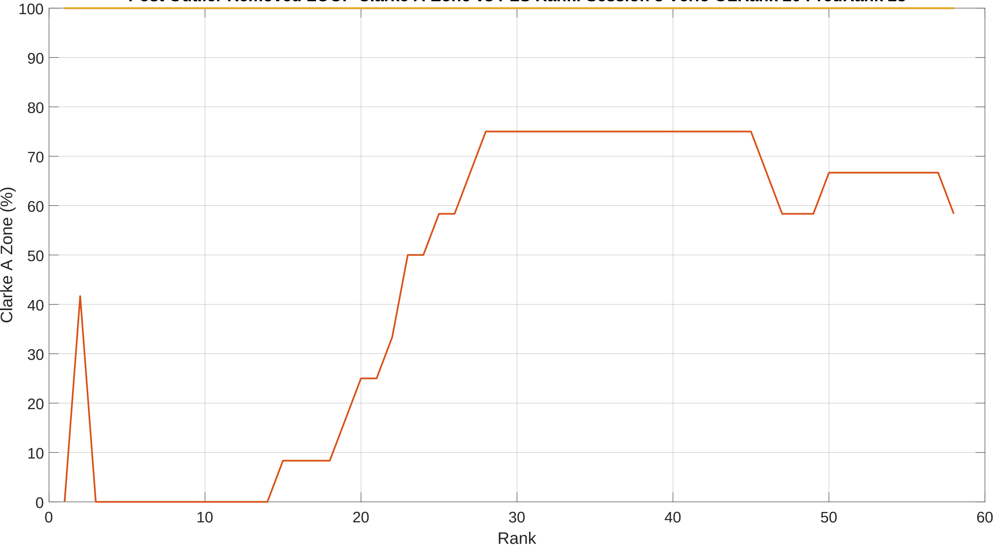
Post Outlier Removed LOOP Clarke A-Zone vs PLS Rank: Session 8 Verio OLRank 20 PredRank 28
