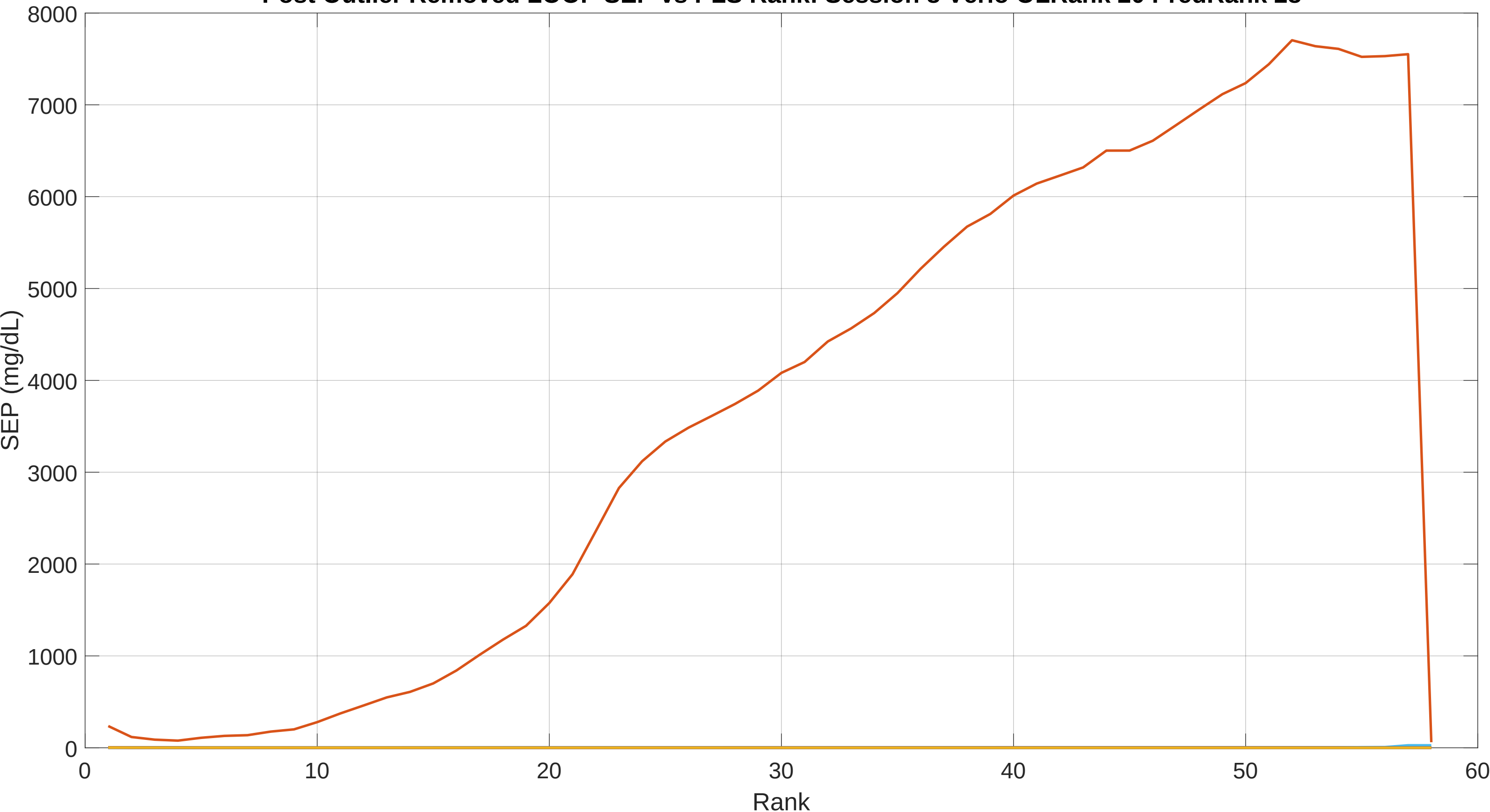
Post Outlier Removed LOOP SEP vs PLS Rank: Session 8 Verio OLRank 20 PredRank 28
