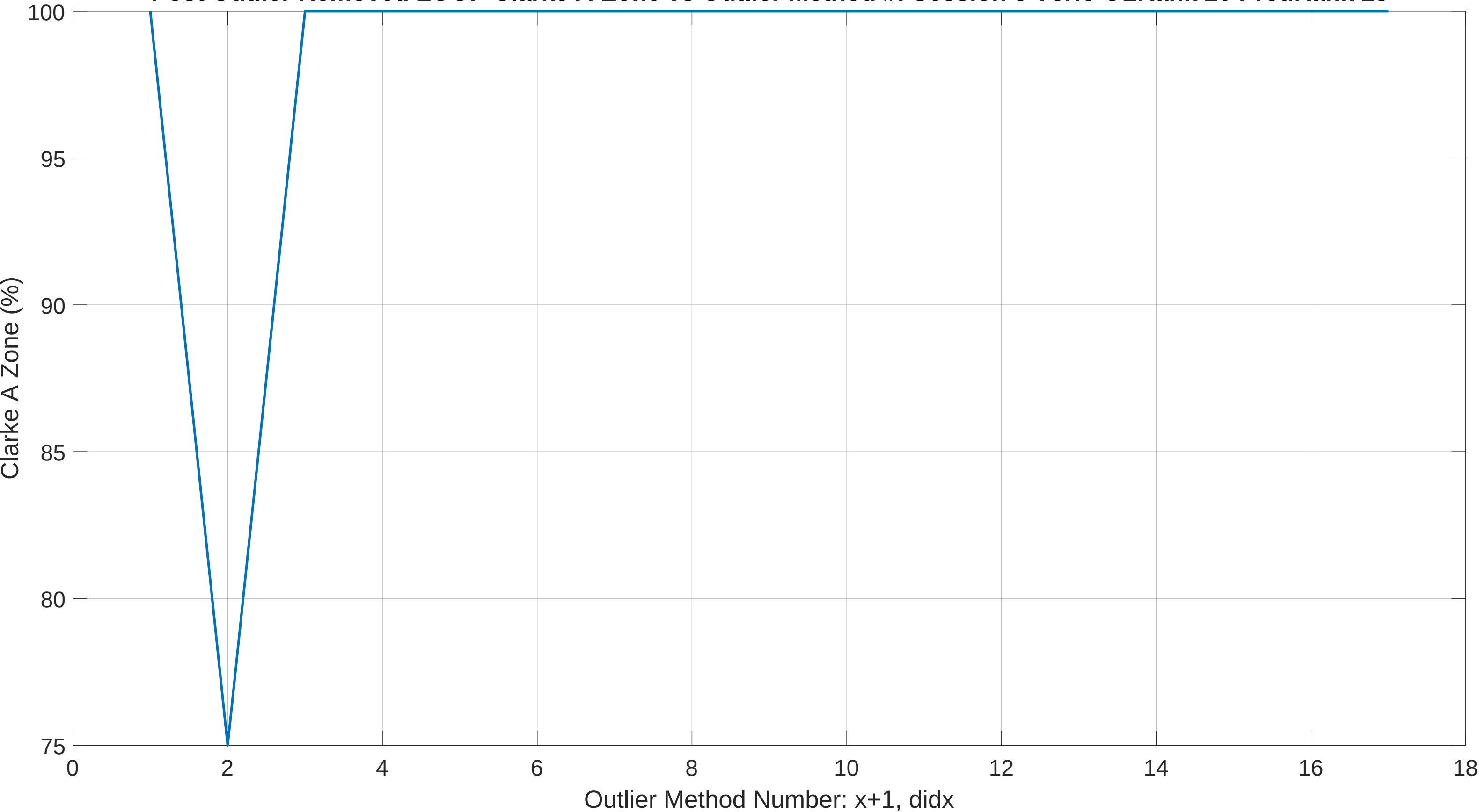
Post Outlier Removed LOOP Clarke A-Zone vs Outlier Method #: Session 8 Verio OLRank 20 PredRank 28
