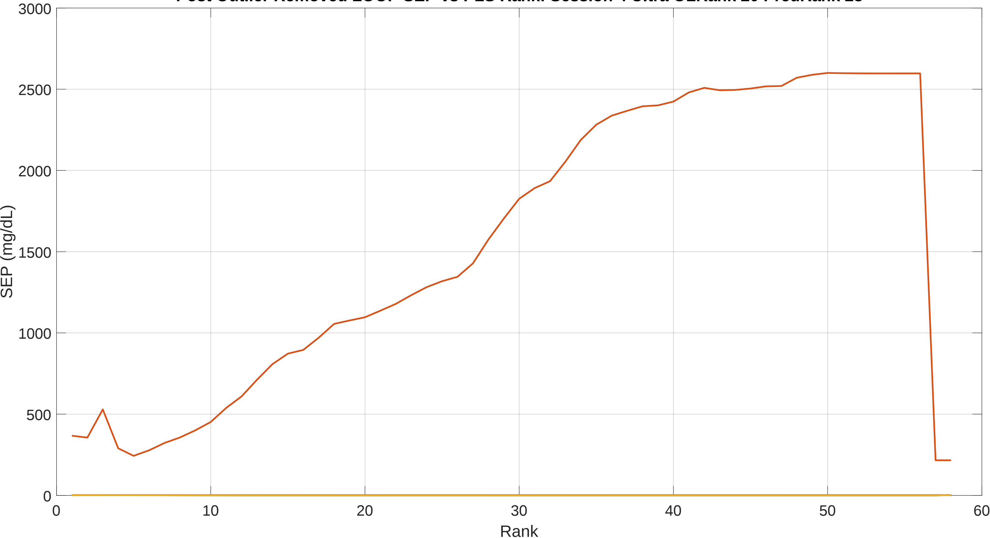
Post Outlier Removed LOOP SEP vs PLS Rank: Session 4 Ultra OLRank 20 PredRank 28
