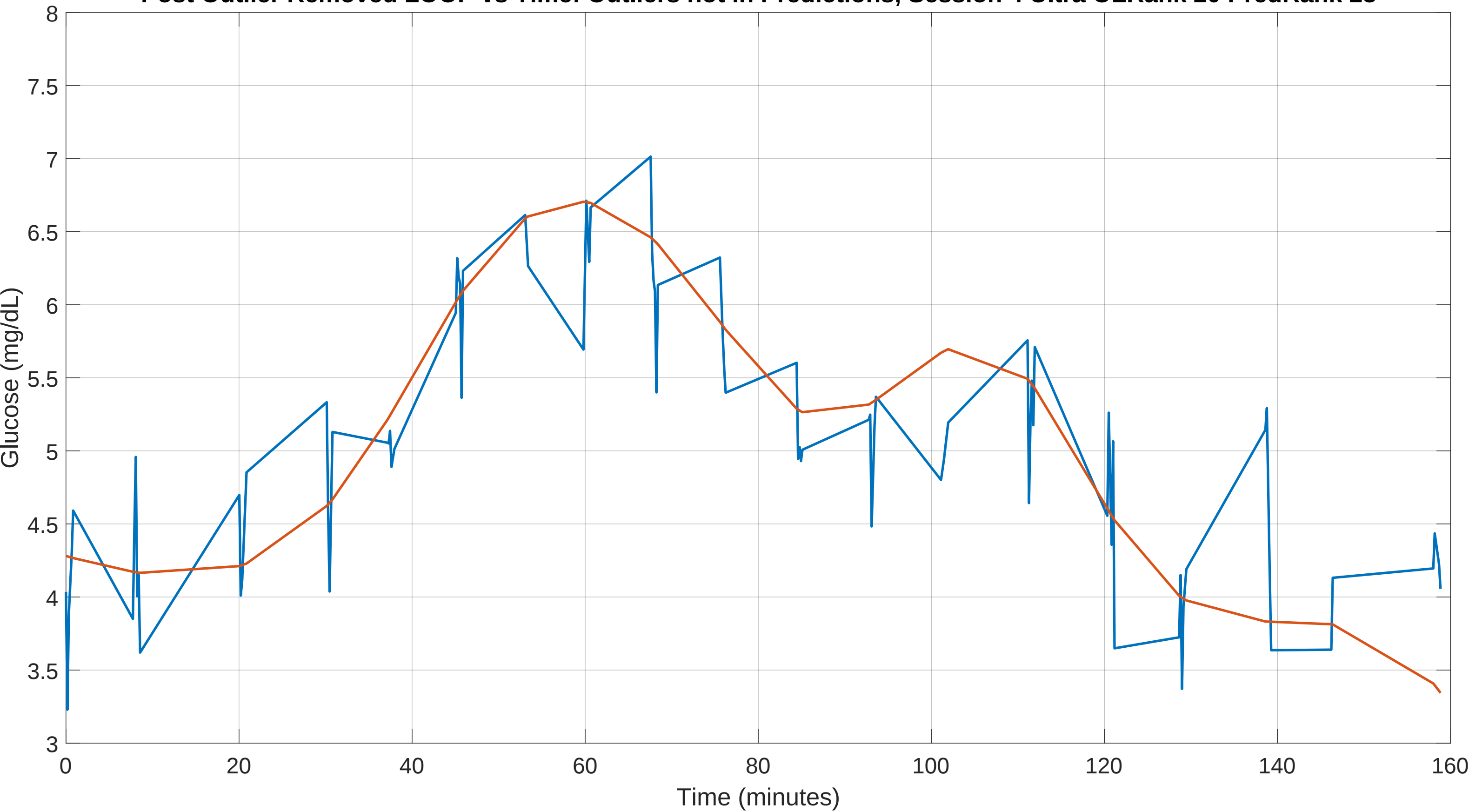
Post Outlier Removed LOOP vs Time: Outliers not in Predictions, Session 4 Ultra OLRank 20 PredRank 28
