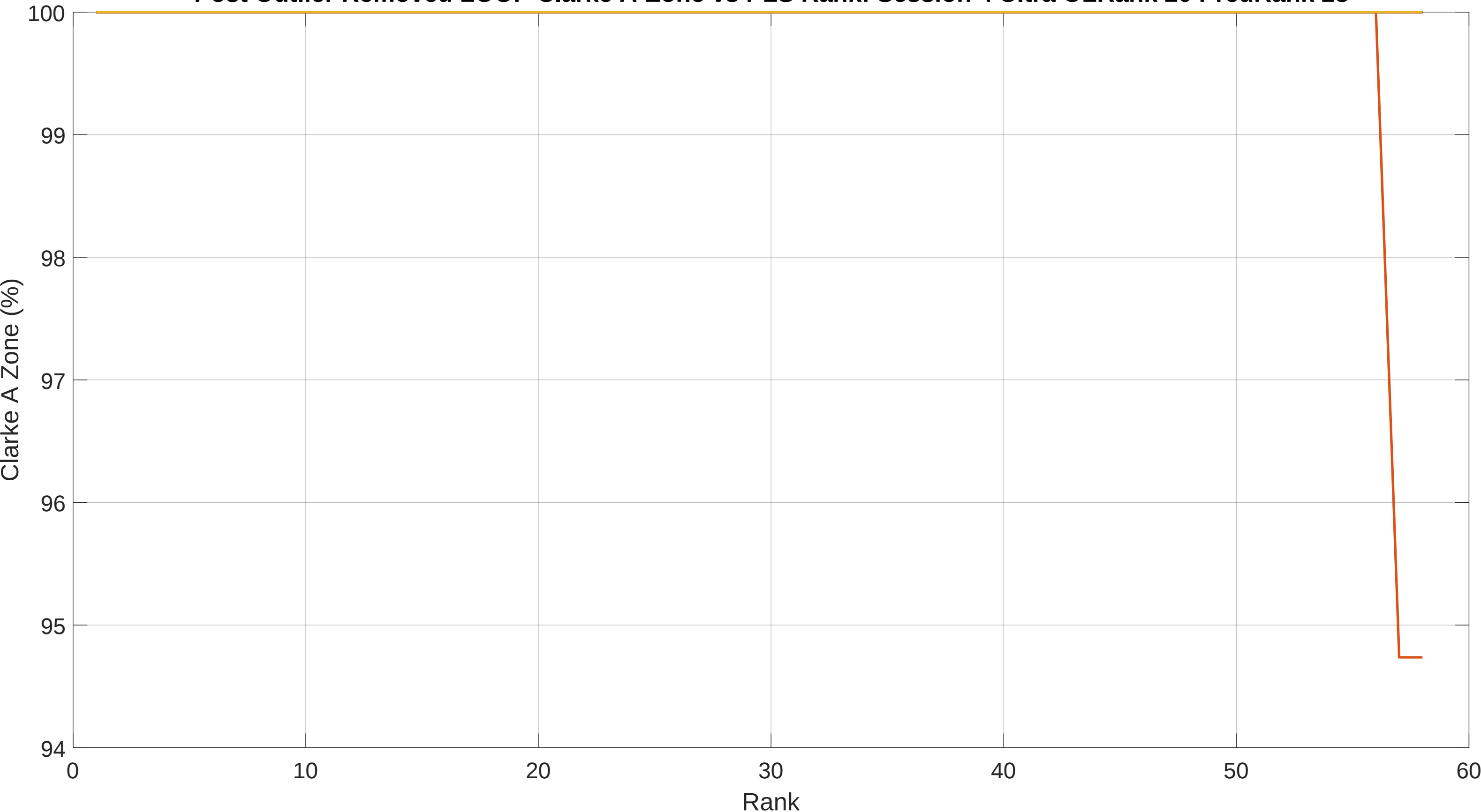
Post Outlier Removed LOOP Clarke A-Zone vs PLS Rank: Session 4 Ultra OLRank 20 PredRank 28
