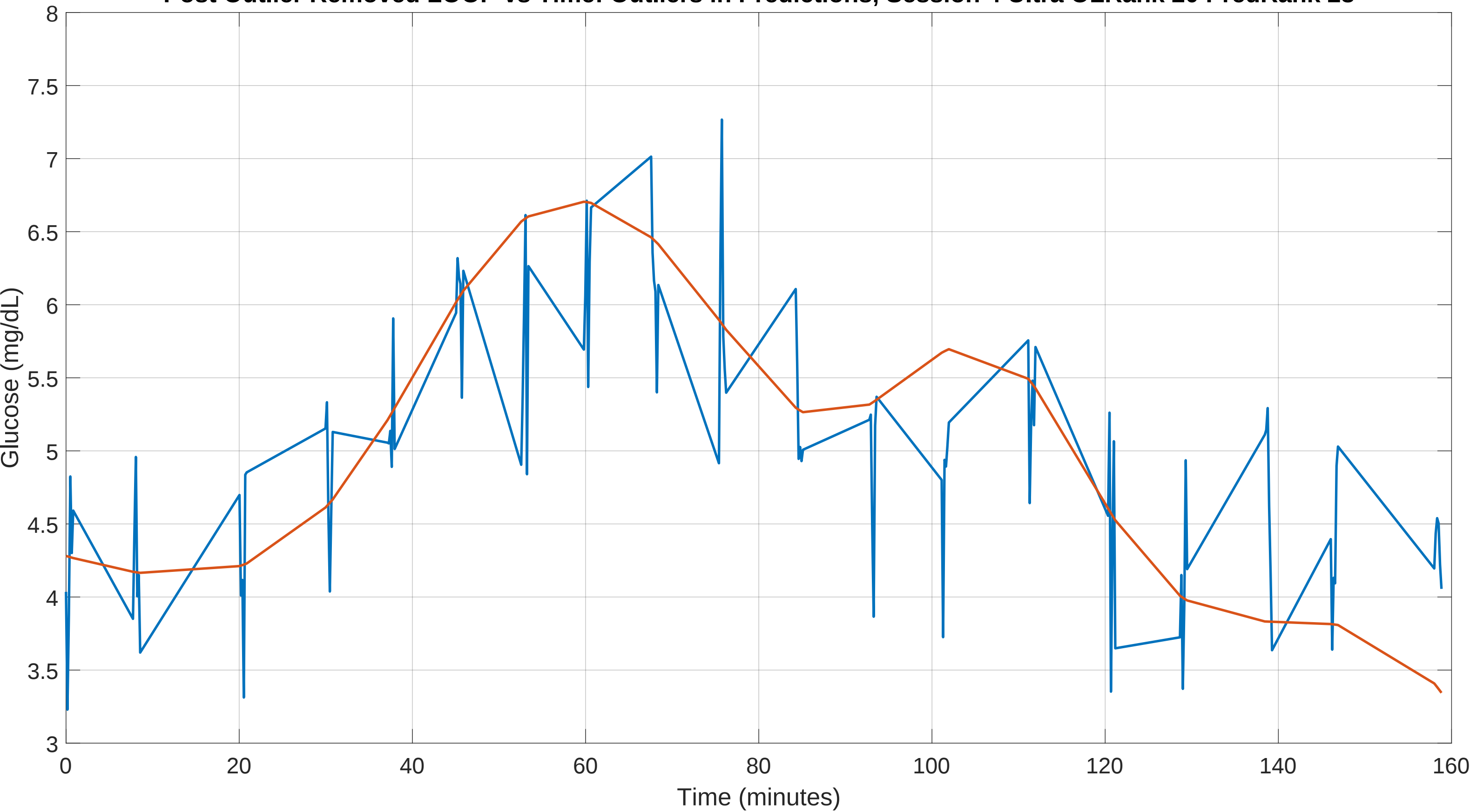
Post Outlier Removed LOOP vs Time: Outliers in Predictions, Session 4 Ultra OLRank 20 PredRank 28
