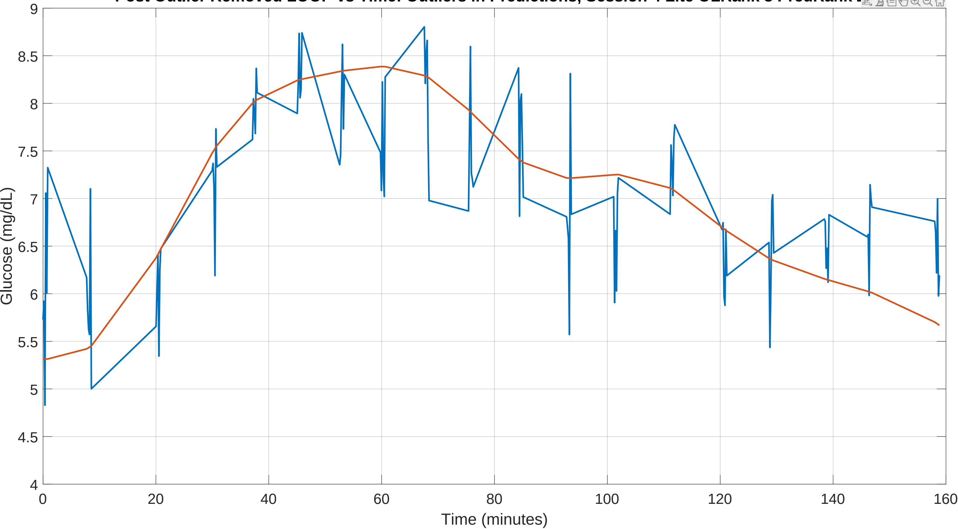
Post Outlier Removed LOOP vs Time: Outliers in Predictions, Session 4 Lite OLRank 8 PredRank 20
