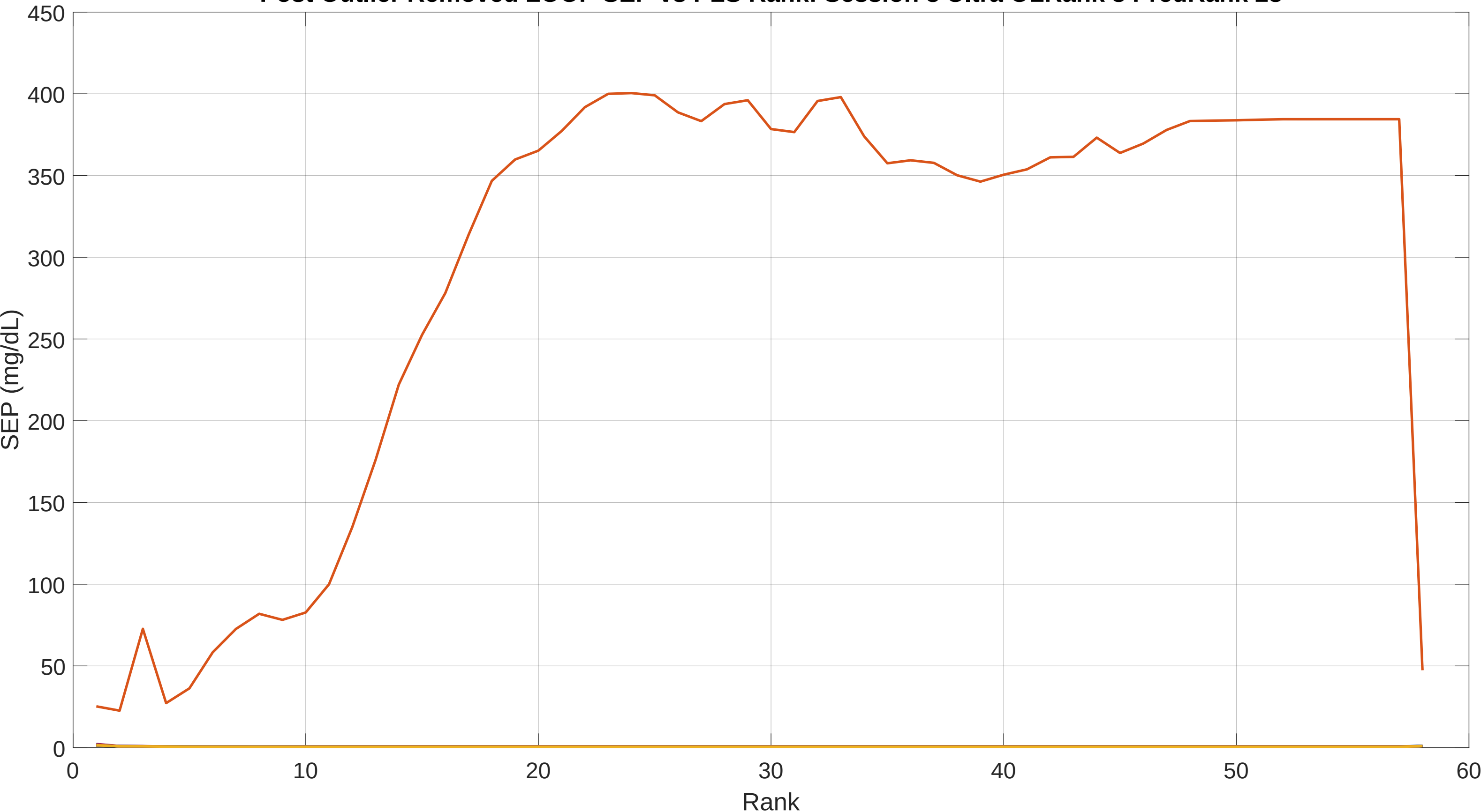
Post Outlier Removed LOOP SEP vs PLS Rank: Session 3 Ultra OLRank 8 PredRank 28
