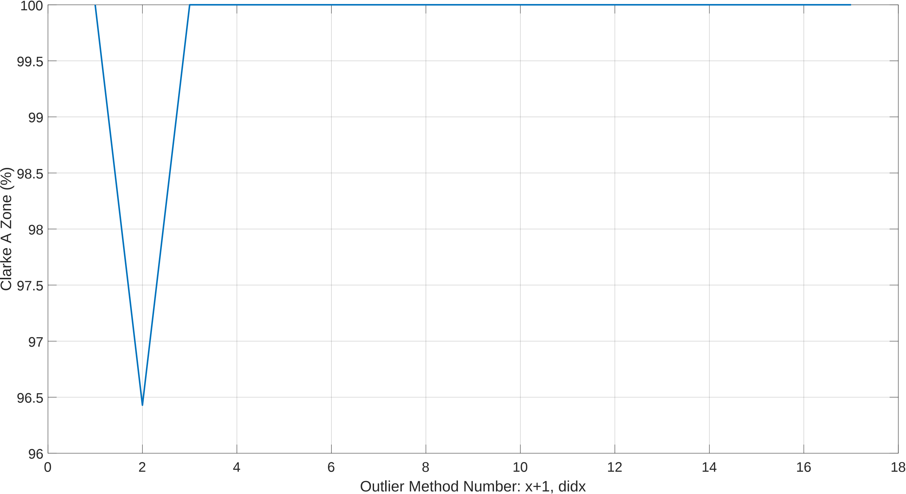
Post Outlier Removed LOOP Clarke A-Zone vs Outlier Method #: Session 1 Ultra OLRank 8 PredRank 28
