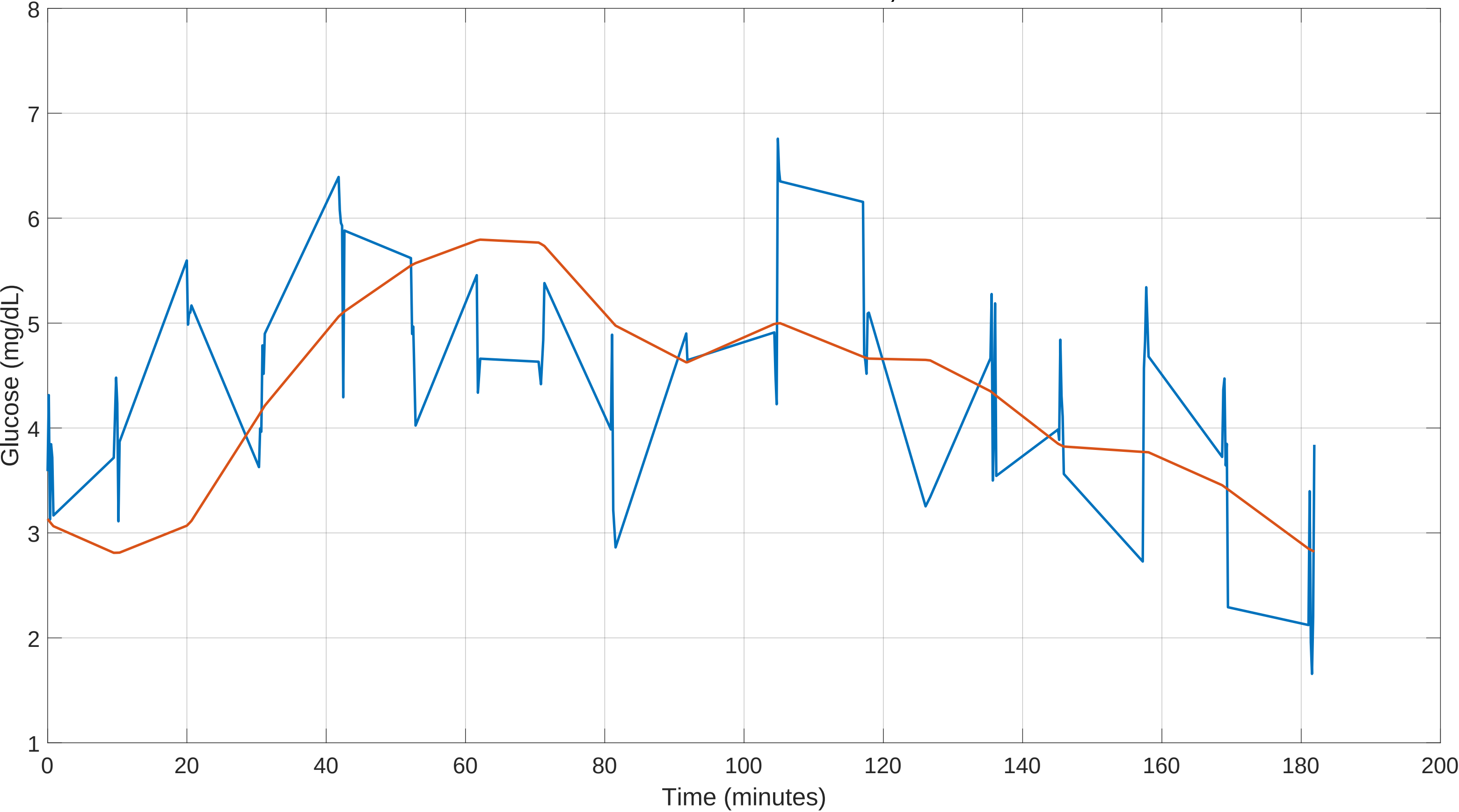
Post Outlier Removed LOOP vs Time: Outliers not in Predictions, Session 12 Oxi OLRank 4 PredRank 28
