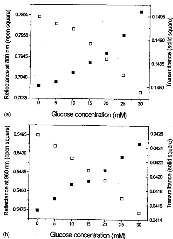
Fig. 1 Effect of glucose concentration on total reflectance ( \square ) and transmittance ( \blacksquare ) at (a) 800 nm and (b) 960 nm.
